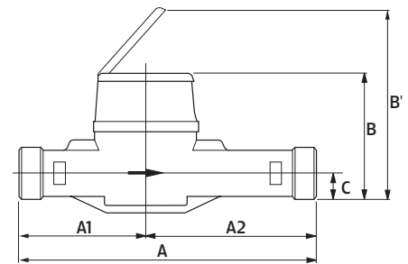
DN 15
